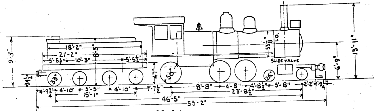
CLASS G-1 ENGS. NOS. 1807-1808
