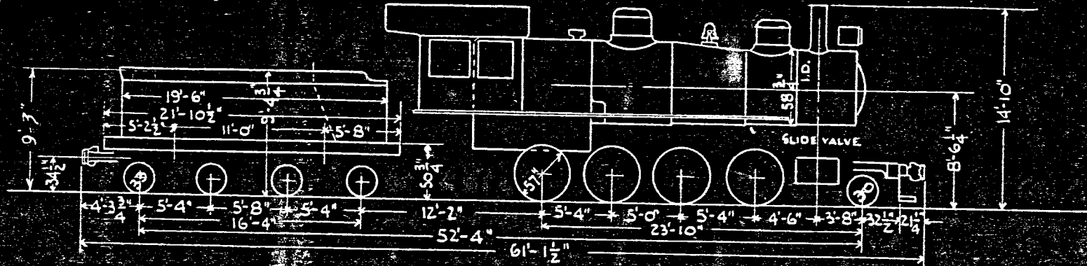
CLASS H-3 ENG. NO. 3011
