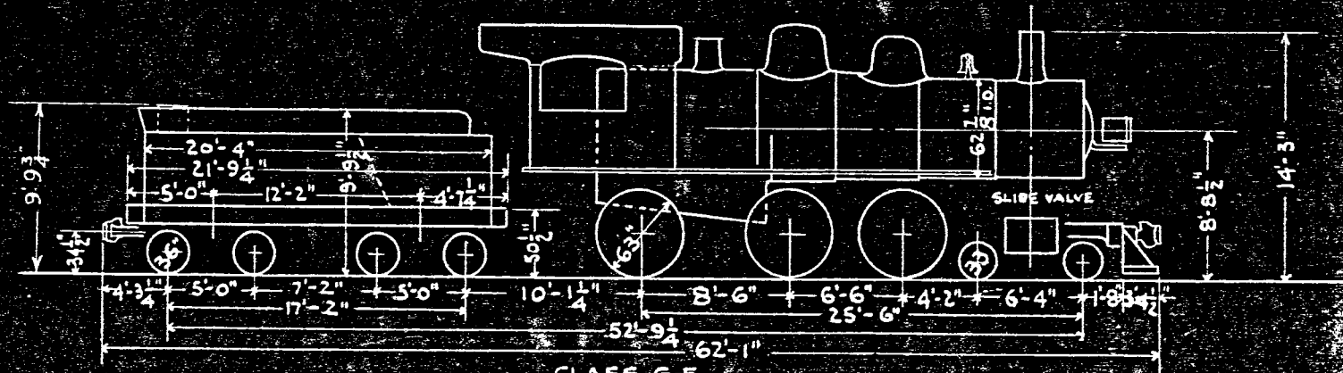
CLASS G-5 ENG. No 2751
