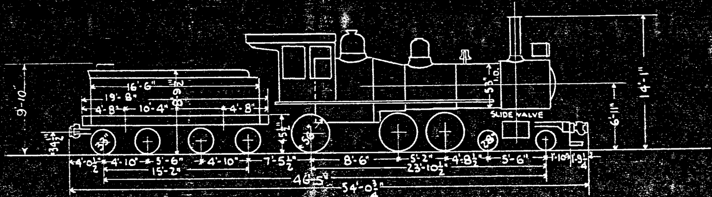
CLASS G-2 ENGS. NOS. 1809-1810
