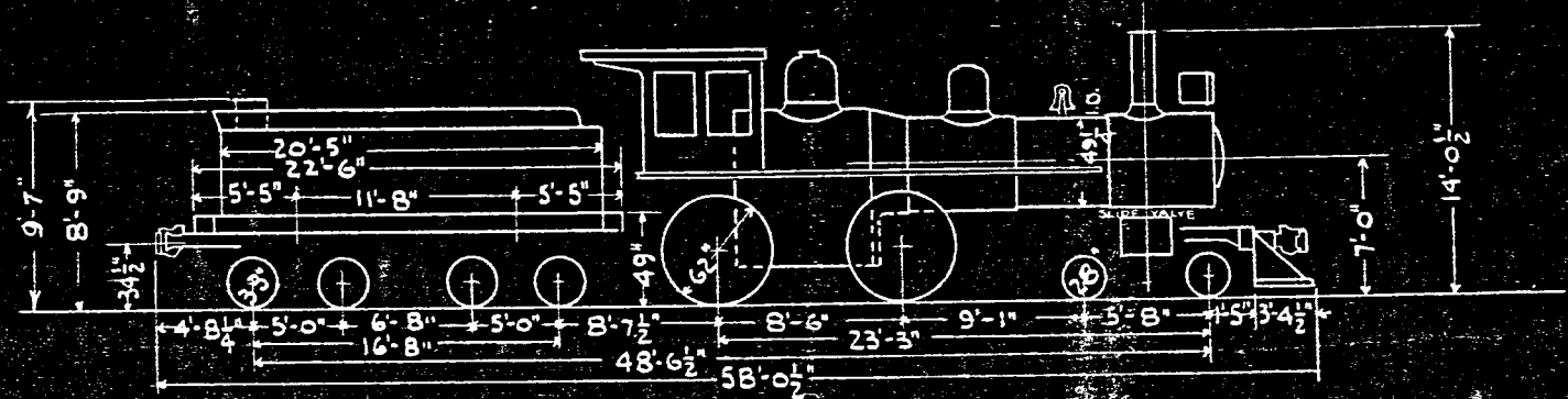
CLASS D-3 ENG. NO 1403
